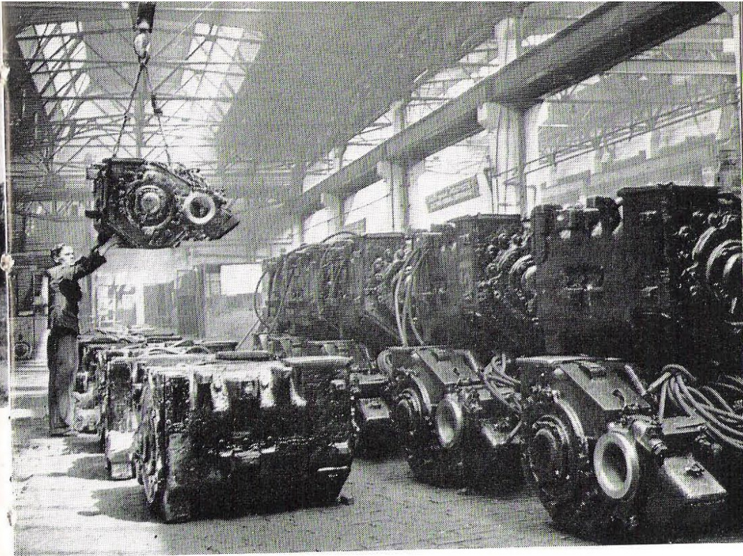
Stacking finished units at the Riga Electrical Machinery Factory, Riga.
