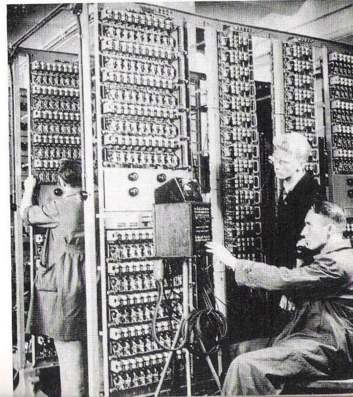
On the right, electrical workers are assembling an automatic telephone exchange at the V.E.F. Factory, Riga.
